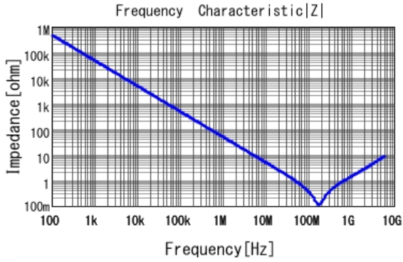
■ GRM033R71E332MA12 |Z| DCOV, 25degC
