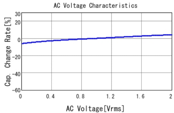
■ GRM033R71E332MA12 C-AC Voltage capchange, DCOV, 25.0d
