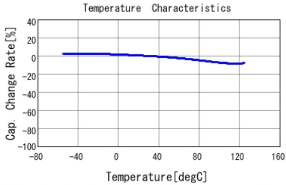
■ GRM033R71E332MA12 C-Temp. capchange, DC0.0V, AC1.0Vrm
