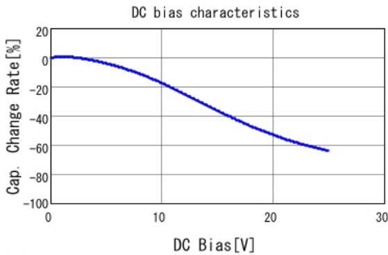
■ GRM033R71E332MA12 C-DC bias capchange, 25.0degC, AC1.
