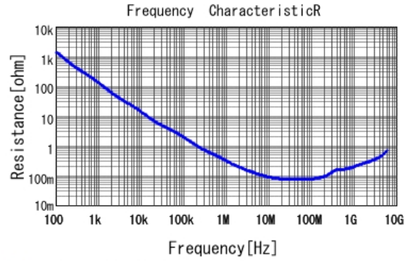
■ GRM033R71C682ME14 R DCOV, 25degC
