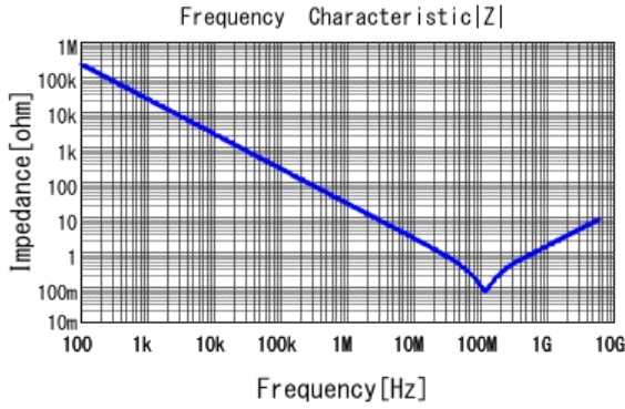
■ GRM033R71C682ME14 |Z| DCOV, 25degC
