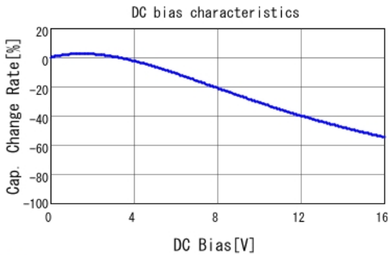
■ GRM033R71C682ME14 C-DC bias capchange, 25.0degC, AC1.
