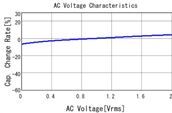
■ GRM033R71C682ME14 C-AC Voltage capchange, DCOV, 25.0d
