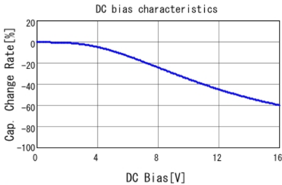
■ GRM033R71C472KE14 C-DC bias capchange, 25.0degC, AC1.
