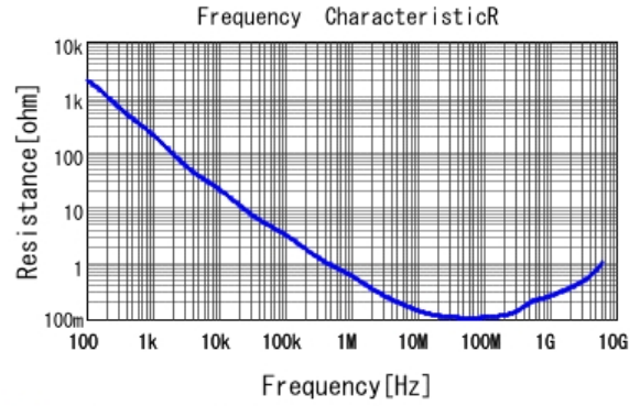
■ GRM033R71C472KE14 R DCOV, 25degC
