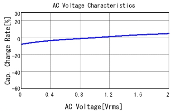
■ GRM033R71C472KE14 C-AC Voltage capchange, DCOV, 25.0d
