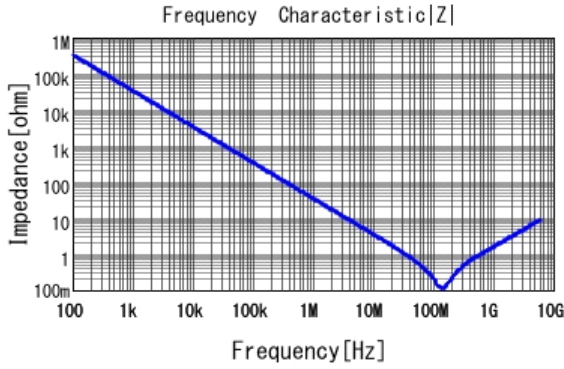
■ GRM033R71C472KE14 |Z| DCOV, 25degC
