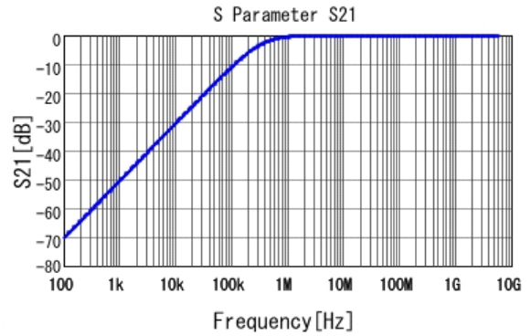
■ GRM033R71C472KE14 S21 DC0V, 25degC
