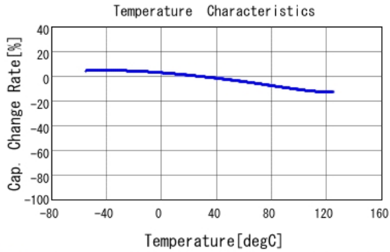
■ GRM033R71C472KE14 C-Temp. capchange, DC0.0V, AC1.0V rm
