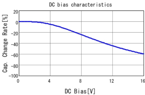
■ GRM033R71C103ME14 C-DC bias capchange, 25.0degC, AC1.
