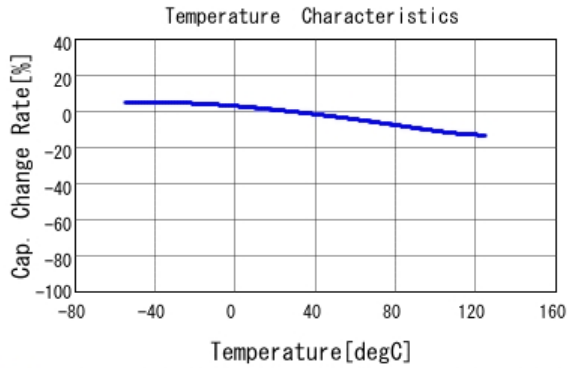
■ GRM033R71C103ME14 C-Temp. capchange, DC0.0V, AC1.0Vrm
