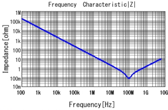
■ GRM033R71C103ME14 |Z| DCOV, 25degC
