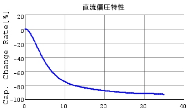
GRM033R6YA104ME14 C-DC bias capchange, 25.0c
