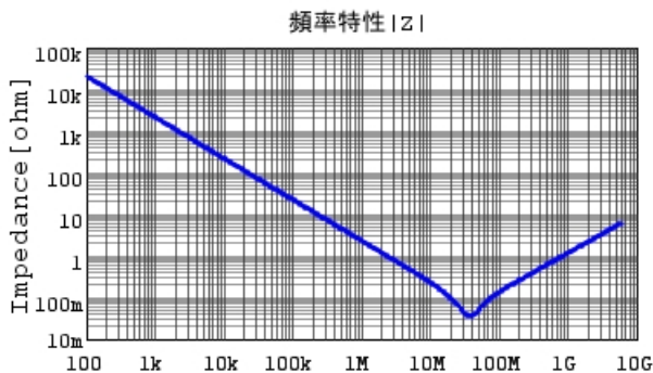
GRM033R6YA104ME14 |Z| DCOV, 25degC
