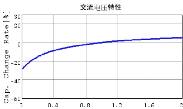
GRM033R6YA104ME14 C-AC Voltage capchange, DC
