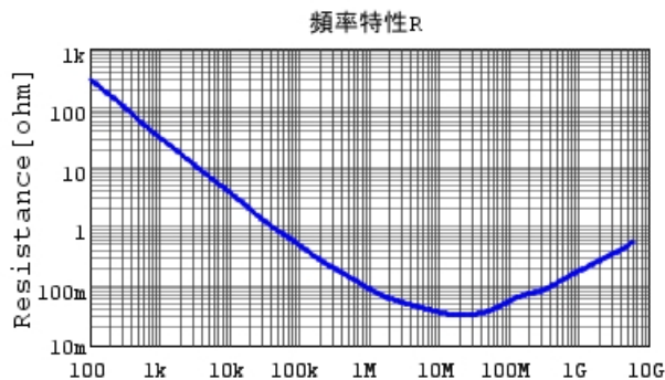
GRM033R6YA104ME14 R DCOV, 25degC
