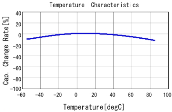
■ GRM033R61C224KE14 C-Temp. capchange, DC0.0V, AC0.2Vrm
