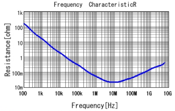
■ GRM033R61C224KE14 R DCOV, 25degC
