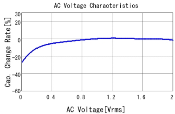
■ GRM033R61C224KE14 C-AC Voltage capchange, DCOV, 25.0d
