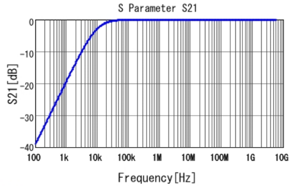
■ GRM033R61C224KE14 S21 DC0V, 25degC
