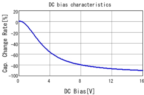
■ GRM033R61C224KE14 C-DC bias capchange, 25.0degC, AC1V
