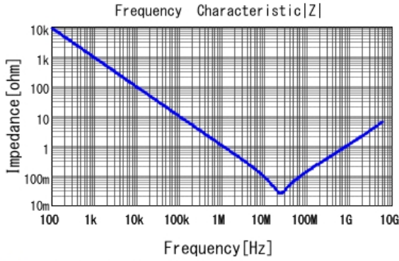
■ GRM033R61C224KE14 |Z| DCOV, 25degC
