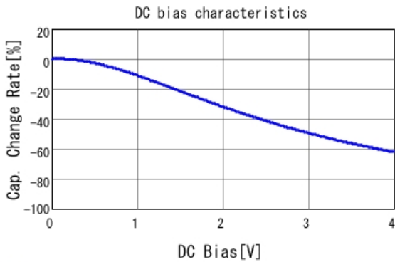
■ GRM033C80G224ME15 C-DC bias capchange, 25.0degC, ACO.
