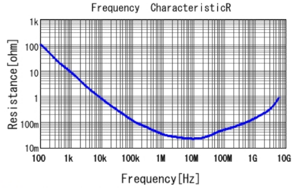
■ GRM033C80G224ME15 R DCOV, 25degC
