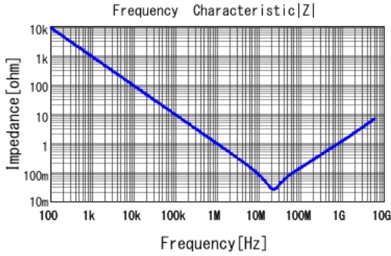
■ GRM033C80G224ME15 |Z| DCOV, 25degC
