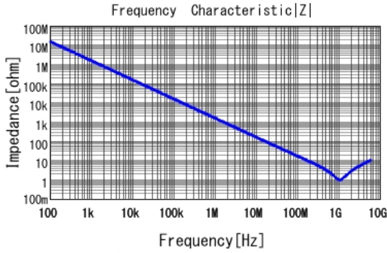
■ GRM033B11E101KA01 |Z| DCOV, 20degC
