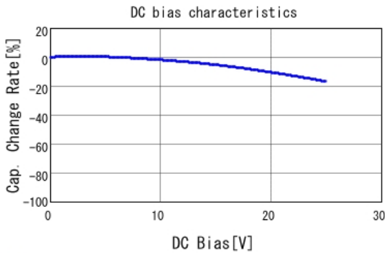
■ GRM033B11E101KA01 C-DC bias capchange, 20.0degC, AC1.
