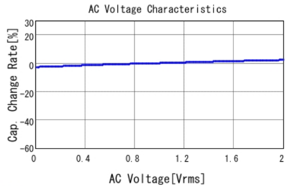
■ GRM033B11E101KA01 C-AC Voltage capchange, DCOV, 20.0d
