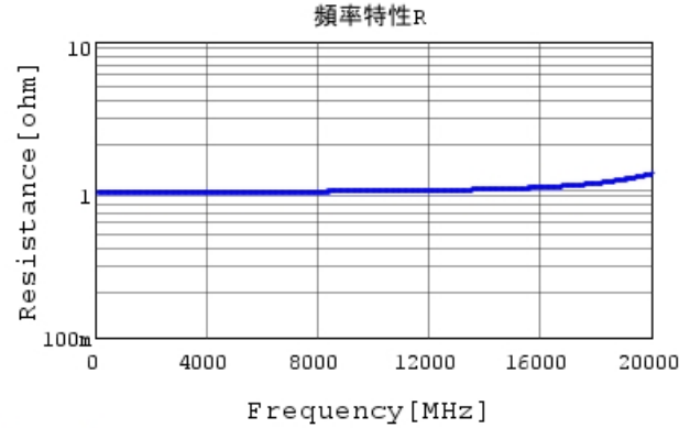
GRM0335C1HR30WA01 R DCOV, 25degC
