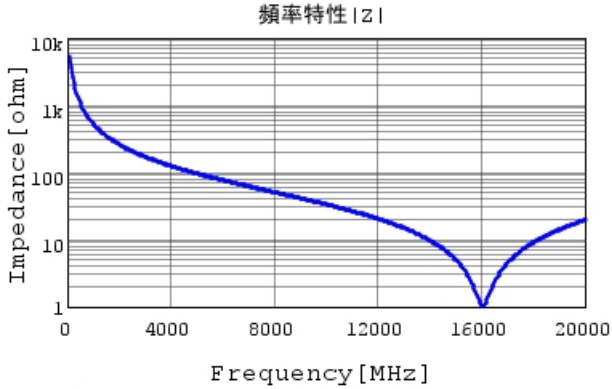
GRM0335C1HR30BA01 |Z| DCOV, 25degC
