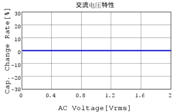
GRM0335C1HR30BA01 C-AC Voltage capchange, DC
