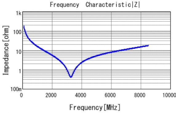
■ GRM0335C1H9R1BA01 |Z| DCOV, 25degC
