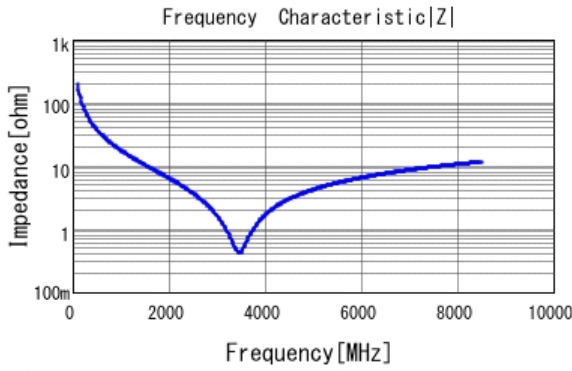
■ GRM0335C1H8R2CA01 |Z| DCOV, 25degC
