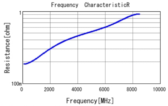
■ GRM0335C1H8R2CA01 R DCOV, 25degC
