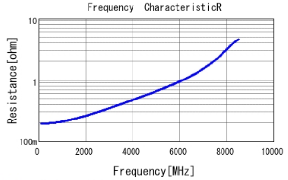
■ GRM0335C1H6R8WA01 R DCOV, 25degC
