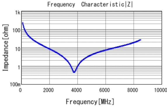
■ GRM0335C1H6R8WA01 |Z| DCOV, 25degC
