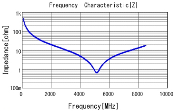
■ GRM0335C1H3R6CA01 |Z| DCOV, 25degC
