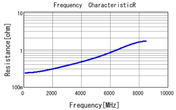
■ GRM0335C1H3R6CA01 R DCOV, 25degC
