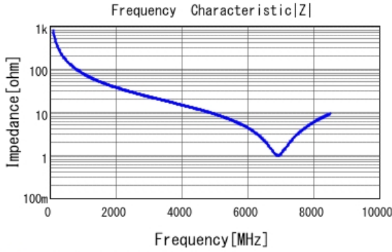
■ GRM0335C1H2R0CA01 |Z| DCOV, 25degC
