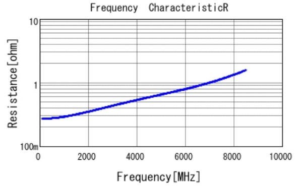
■ GRM0335C1H2R0CA01 R DCOV, 25degC
