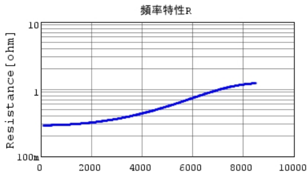
GRM0335C1H1R6BA01 R DCOV, 25degC
