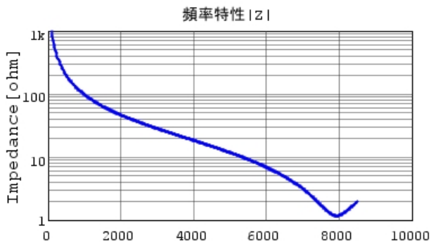
GRM0335C1H1R6BA01 |Z| DCOV, 25degC
