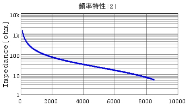
GRM0335C1H1R1BA01 |Z| DCOV, 25degC
