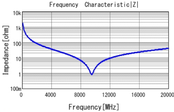
■ GRM0334C2AR90BA01 |Z| DCOV, 20degC
