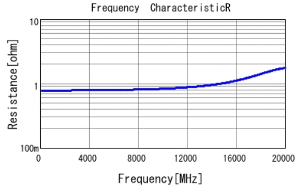
■ GRM0334C2AR90BA01 R DCOV, 20degC
