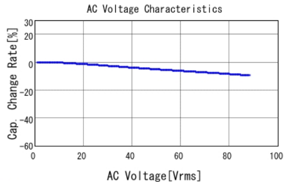
■ GRJ43DR72E474KWJ1 C-AC Voltage capchange, DC0V, 25.0d
