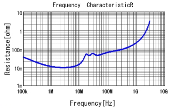
■ GRJ43DR72E474KWJ1 R DC0V, 25degC
