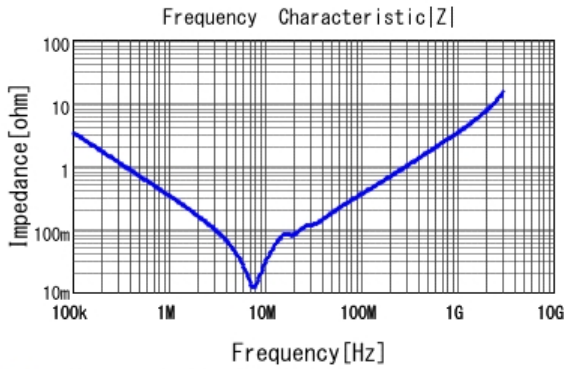
■ GRJ43DR72E474KWJ1 |Z| DC0V, 25degC
