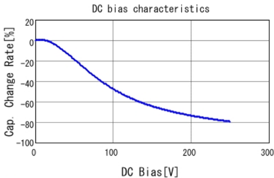
■ GRJ43DR72E474KWJ1 C-DC bias capchange, 25.0degC, AC1V
