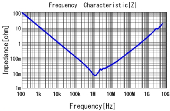
■ GRJ32ER71C226KE11 |Z| DCOV, 25degC
