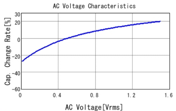
■ GRJ32ER71C226KE11 C-AC Voltage capchange, DCOV, 25.0d
