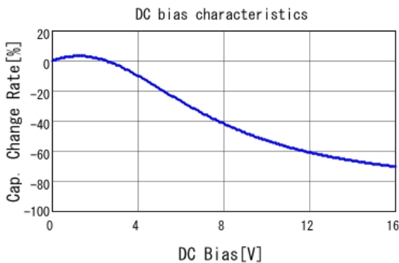
■ GRJ32ER71C226KE11 C-DC bias capchange, 25.0degC, AC0.
