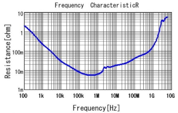
■ GRJ32ER71C226KE11 R DCOV, 25degC
