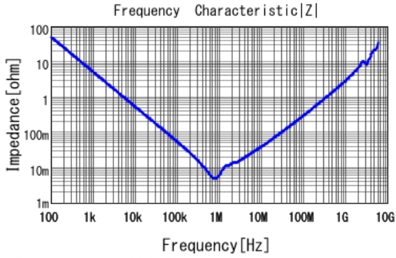
■ GRJ32ER71A476KE11 |Z| DCOV, 25degC
