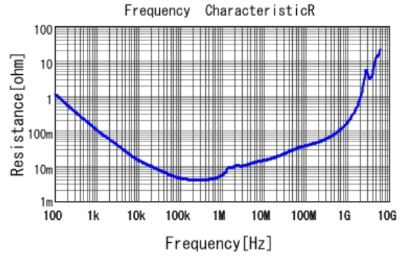
■ GRJ32ER71A476KE11 R DCOV, 25degC
