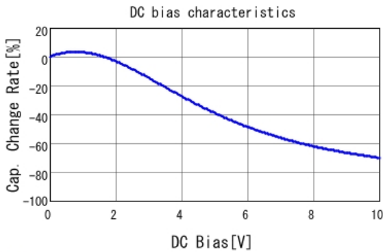
■ GRJ32ER71A476KE11 C-DC bias capchange, 25.0degC, AC0.
