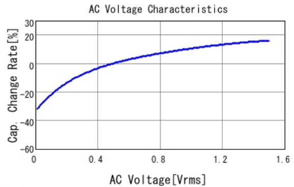
■ GRJ32ER71A476KE11 C-AC Voltage capchange, DCOV, 25.0d
