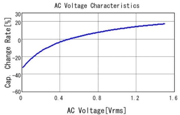
■ GRJ32ER70J476KE11 C-AC Voltage capchange, DCOV, 25.0d
