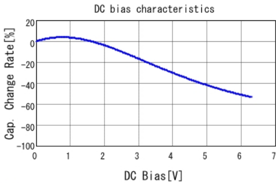
■ GRJ32ER70J476KE11 C-DC bias capchange, 25.0degC, AC0.
