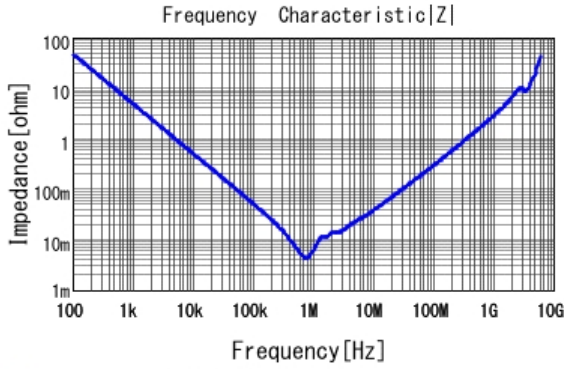
■ GRJ32ER70J476KE11 |Z| DCOV, 25degC
