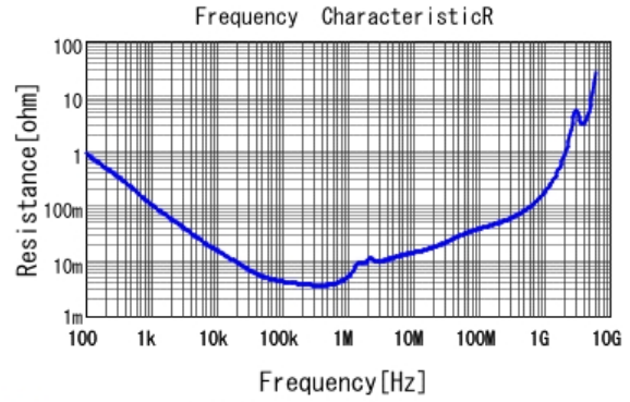
■ GRJ32ER70J476KE11 R DCOV, 25degC
