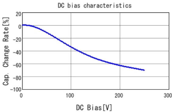
■ GRJ21AR72E472KWJ1 C-DC bias capchange, 25.0degC, AC1V
