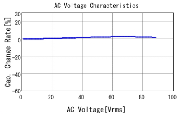
■ GRJ21AR72E472KWJ1 C-AC Voltage capchange, DCOV, 25.0d
