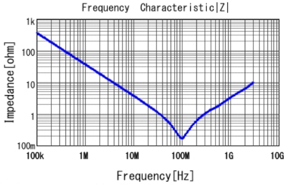
■ GRJ21AR72E472KWJ1 |Z| DCOV, 25degC
