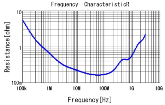
■ GRJ21AR72E472KWJ1 R DCOV, 25degC
