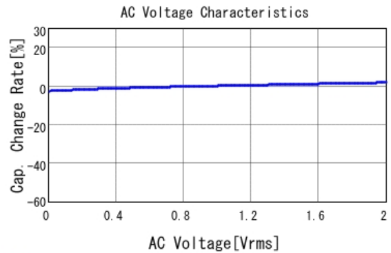
■ GRJ216R71H223KE01 C-AC Voltage capchange, DCOV, 25.0d
