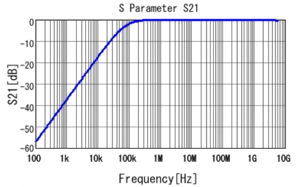
■ GRJ216R71H223KE01 S21 DC0V, 25degC
