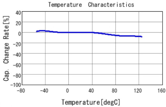
■ GRJ216R71H223KE01 C-Temp. capchange, DC0.0V, AC1.0Vrm
