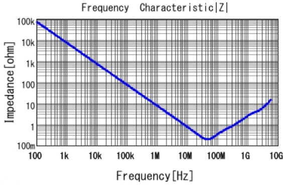
■ GRJ216R71H223KE01 |Z| DCOV, 25degC
