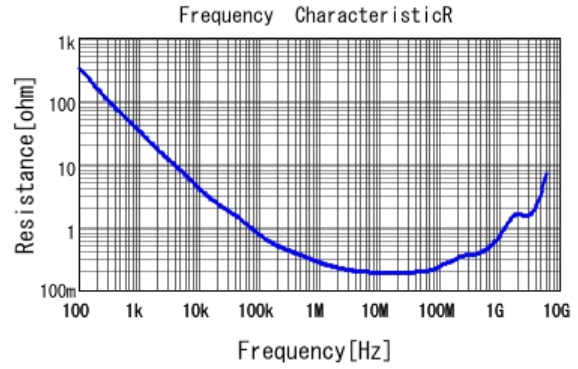
■ GRJ216R71H223KE01 R DCOV, 25degC
