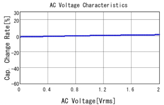
■ GRJ188R72A102KE11 C-AC Voltage capchange, DCOV, 25.0d
