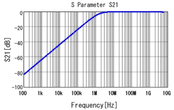
■ GRJ188R72A102KE11 S21 DC0V, 25degC
