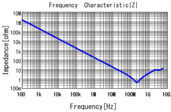
■ GRJ188R72A102KE11 |Z| DCOV, 25degC
