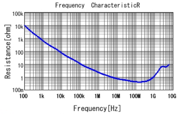
■ GRJ188R72A102KE11 R DCOV, 25degC
