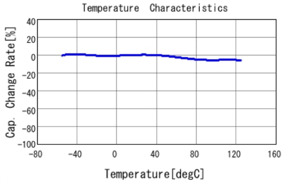
■ GRJ188R72A102KE11 C-Temp. capchange, DC0.0V, AC1.0Vrm
