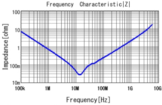
■ GRJ188R71H224KE11 |Z| DCOV, 25degC
