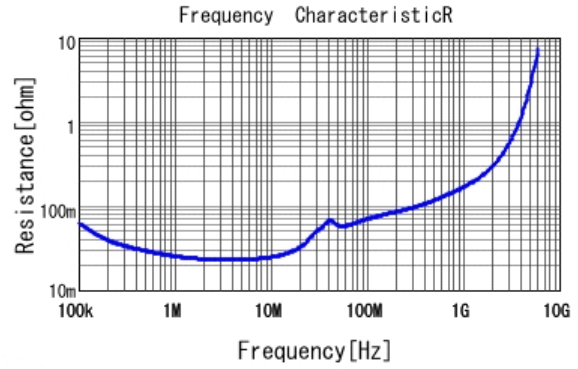
■ GRJ188R71H224KE11 R DCOV, 25degC
