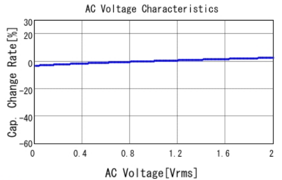
■ GRJ188R71H224KE11 C-AC Voltage capchange, DCOV, 25.0d
