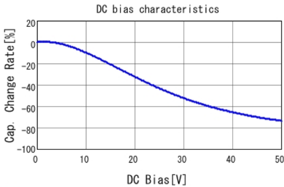
■ GRJ188R71H224KE11 C-DC bias capchange, 25.0degC, AC1.
