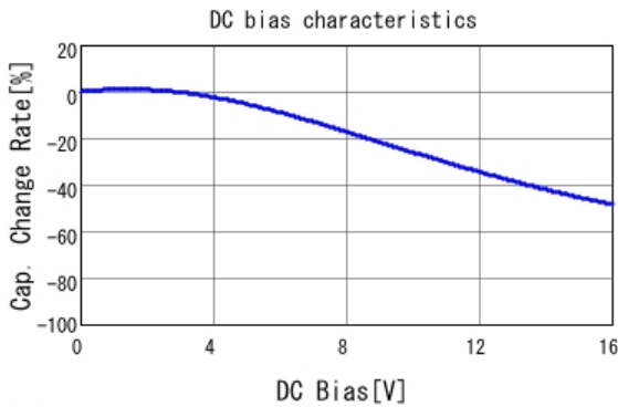
■ GRJ188R71C474KE11 C-DC bias capchange, 25.0degC, AC1.
