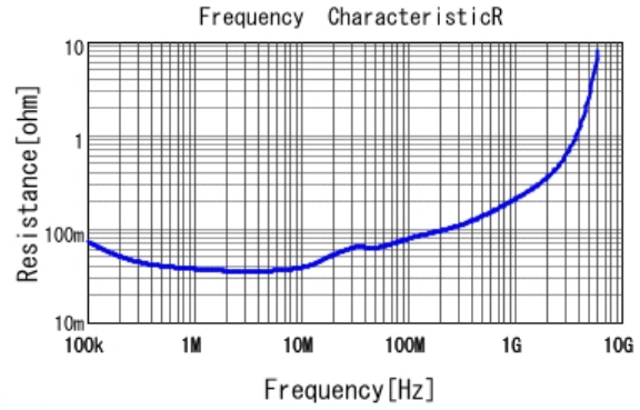
■ GRJ188R71C474KE11 R DCOV, 25degC
