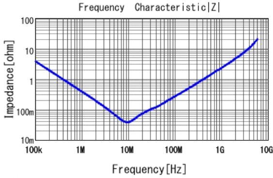
■ GRJ188R71C474KE11 |Z| DCOV, 25degC
