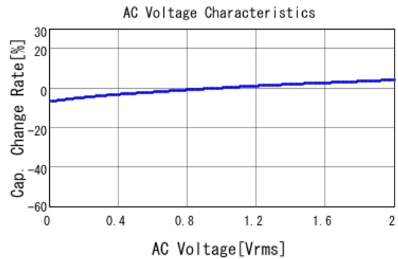
■ GRJ188R71C474KE11 C-AC Voltage capchange, DCOV, 25.0d
