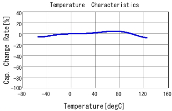
■ GRJ188R70J225KE11 C-Temp. capchange, DC0.0V, AC0.5Vrm
