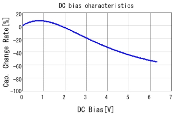
■ GRJ188R70J225KE11 C-DC bias capchange, 25.0degC, AC0.
