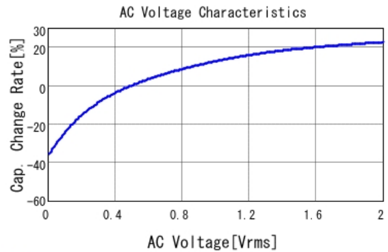
■ GRJ188R70J225KE11 C-AC Voltage capchange, DCOV, 25.0d
