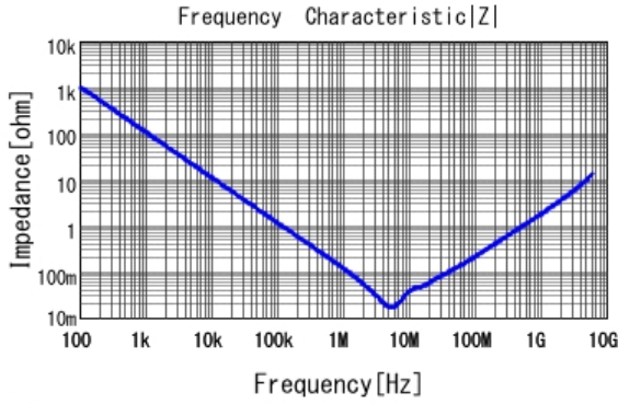
■ GRJ188R70J225KE11 |Z| DCOV, 25degC
