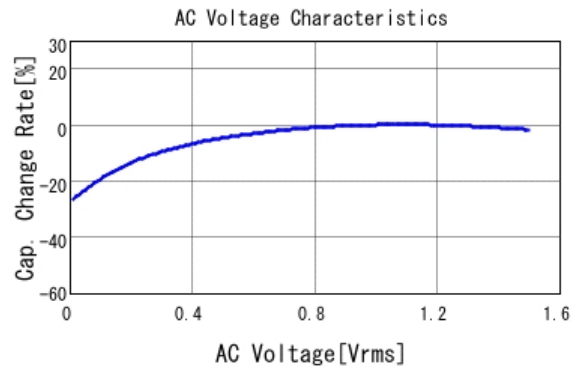
■ GRJ188R60J106ME11 C-AC Voltage capchange, DCOV, 25.0d
