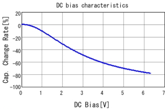
■ GRJ188R60J106ME11 C-DC bias capchange, 25.0degC, AC1V
