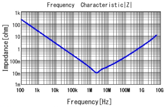
■ GRJ188R60J106ME11 |Z| DCOV, 25degC
