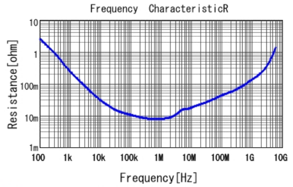
■ GRJ188R60J106ME11 R DCOV, 25degC
