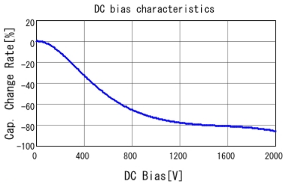
■ GR443QR73D332KW01 C-DC bias capchange, 25.0degC, AC1V
