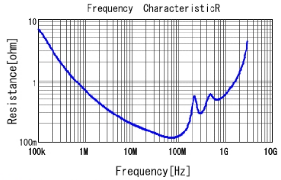
■ GR443QR73D332KW01 R DCOV, 25degC
