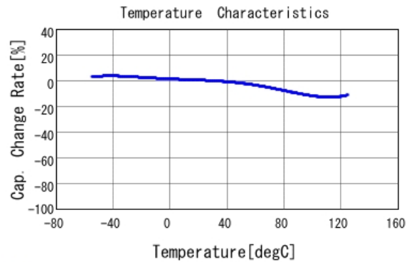
■ GR443QR73D332KW01 C-Temp. capchange, DCOV, AC1Vrms
