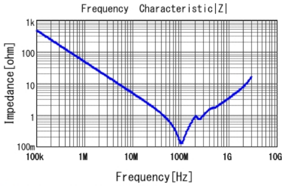
■ GR443QR73D332KW01 |Z| DCOV, 25degC
