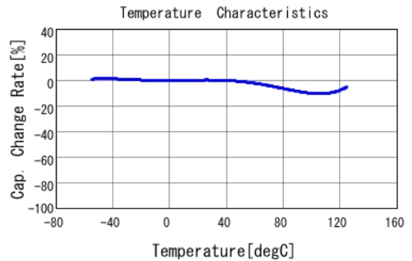
■ GR443QR73D102KW01 C-Temp. capchange, DCOV, AC1Vrms
