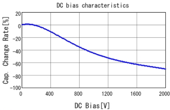
■ GR443QR73D102KW01 C-DC bias capchange, 25.0degC, AC1V
