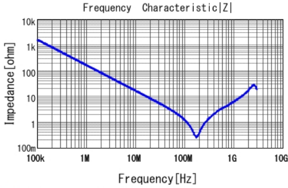
■ GR443QR73D102KW01 |Z| DCOV, 25degC
