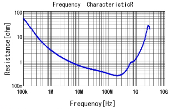
■ GR443QR73D102KW01 R DCOV, 25degC
