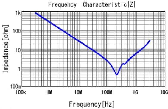
■ GR442QR73D681KW01 |Z| DCOV, 25degC
