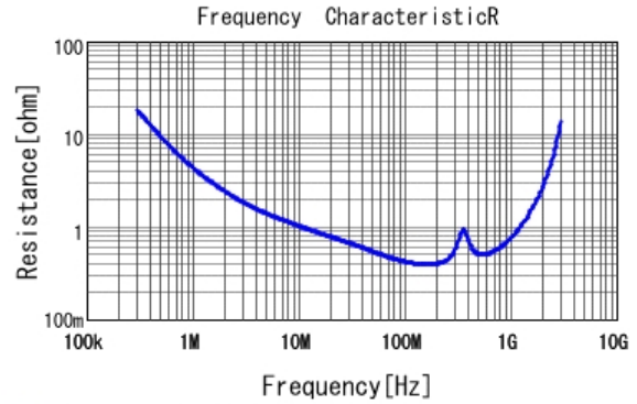
■ GR442QR73D681KW01 R DCOV, 25degC
