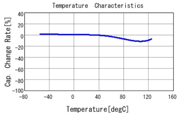
■ GR442QR73D681KW01 C-Temp. capchange, DCOV, AC1Vrms
