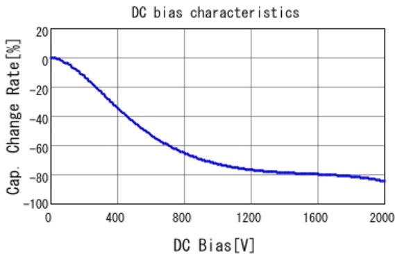
■ GR442QR73D681KW01 C-DC bias capchange, 25.0degC, AC1V
