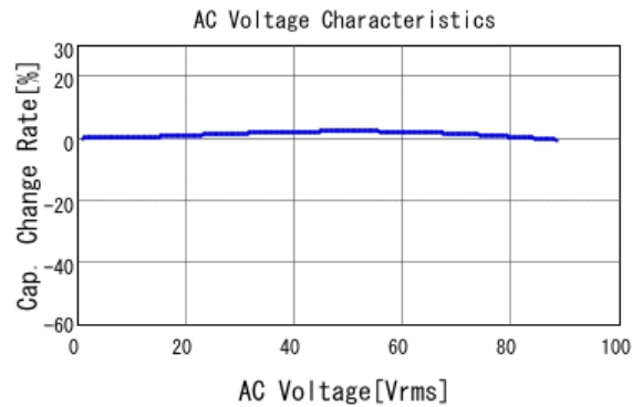
■ GR355DD72E684KW01 C-AC Voltage capchange, DC0V, 25.0d
