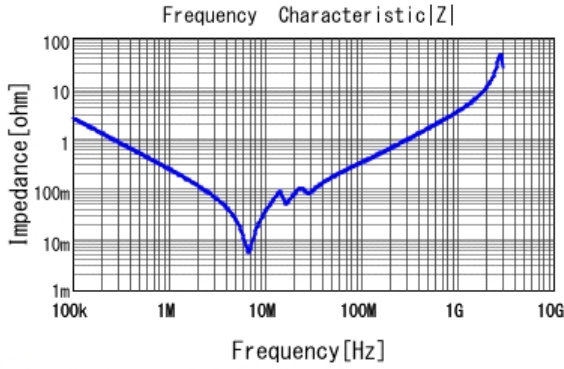
■ GR355DD72E684KW01 |Z| DC0V, 25degC
