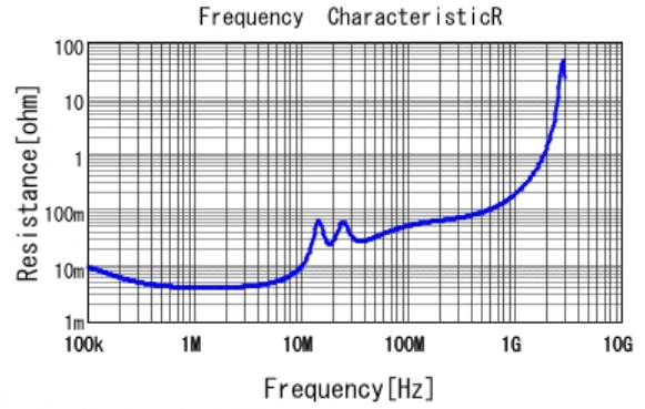
■ GR355DD72E684KW01 R DC0V, 25degC
