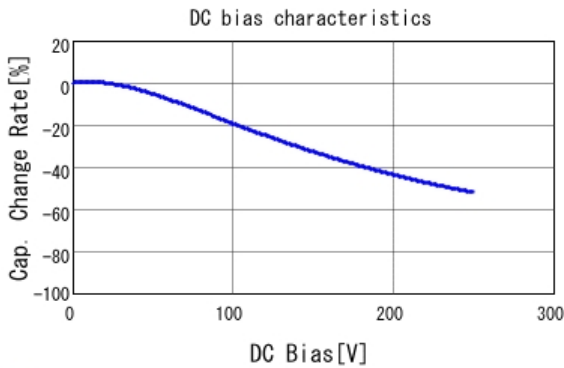
■ GR355DD72E684KW01 C-DC bias capchange, 25.0degC, AC1V
