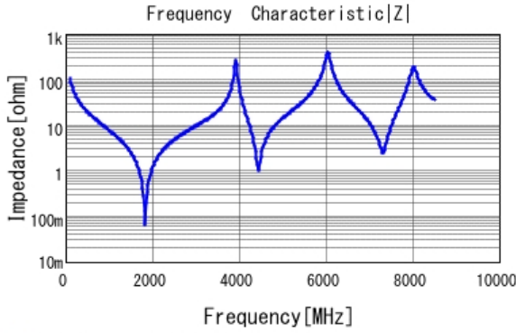
■ GQM22M5C2H150GB01 |Z| DC0V, 25degC
