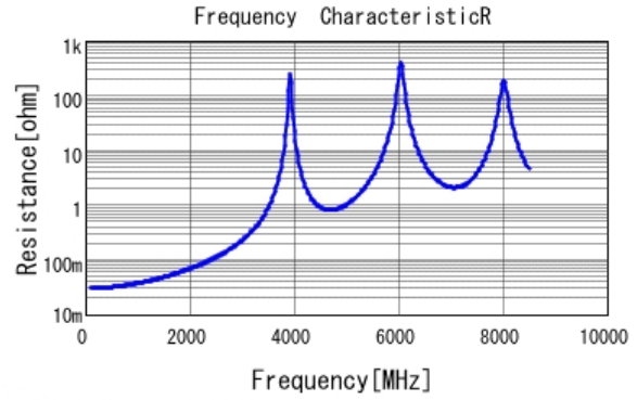
■ GQM22M5C2H150GB01 R DC0V, 25degC
