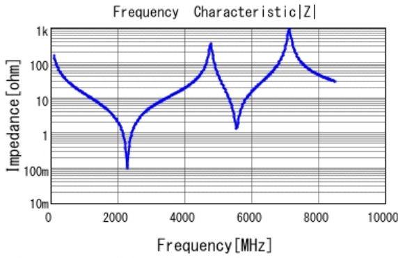
■ GQM22M5C2H100JB01 |Z| DC0V, 25degC
