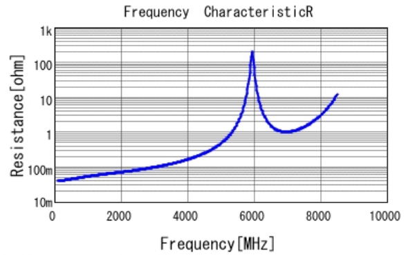
■ GQM2195C2E7R0DB12 R DCOV, 25degC
