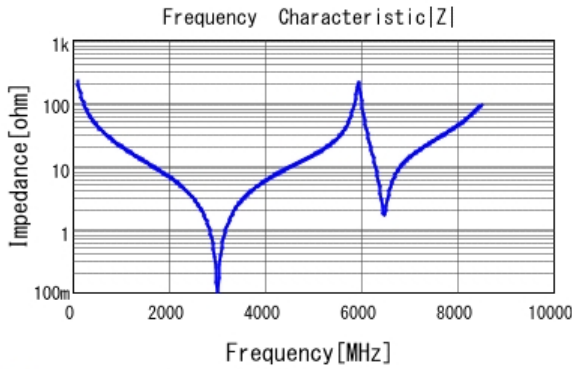
■ GQM2195C2E7R0DB12 |Z| DCOV, 25degC
