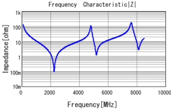
■ GQM2195C2E120JB12 |Z| DC0V, 25degC
