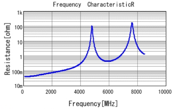
■ GQM2195C2E120JB12 R DC0V, 25degC
