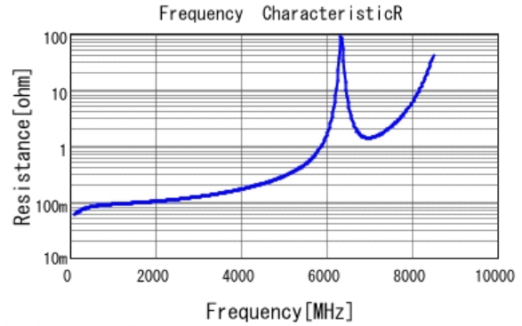
■ GQM2195C2A5R1CB01 R DCOV, 25degC
