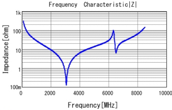
■ GQM2195C2A5R1CB01 |Z| DCOV, 25degC
