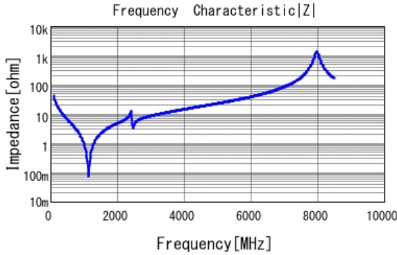
■ GQM2195C1H390JB01 |Z| DCOV, 25degC
