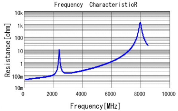
■ GQM2195C1H390JB01 R DCOV, 25degC
