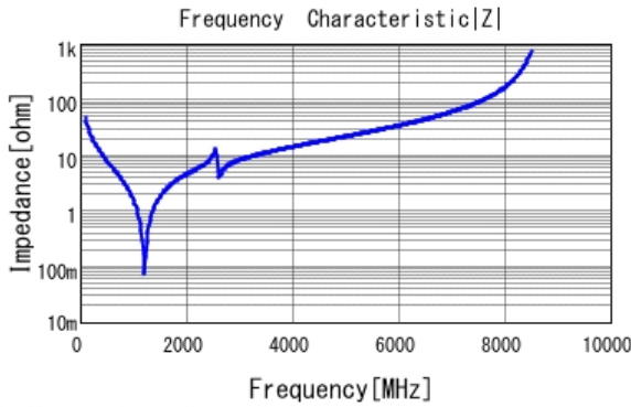
■ GQM2195C1H330JB01 |Z| DCOV, 25degC
