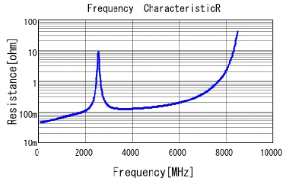
■ GQM2195C1H330JB01 R DCOV, 25degC
