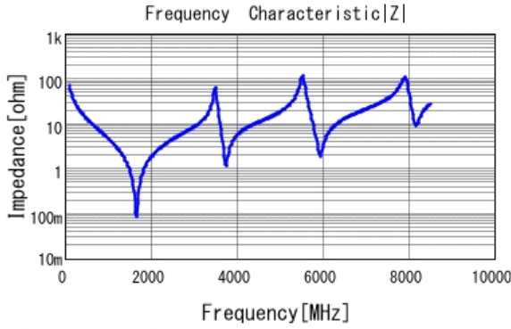
■ GQM2195C1H220JB01 |Z| DCOV, 25degC
