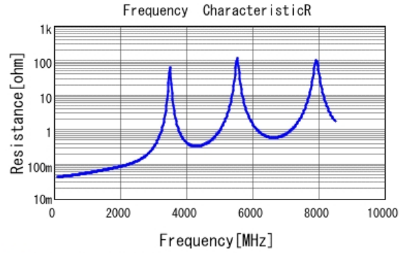
■ GQM2195C1H220JB01 R DCOV, 25degC
