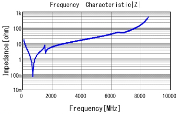
■ GQM2195C1H101JB01 |Z| DCOV, 25degC
