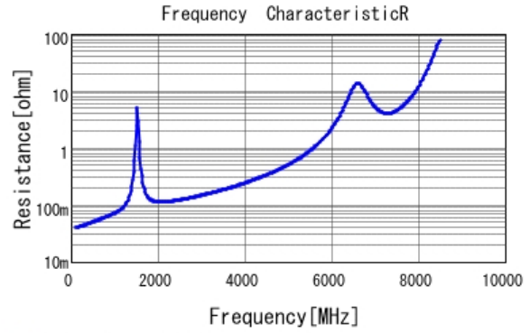
■ GQM2195C1H101JB01 R DCOV, 25degC
