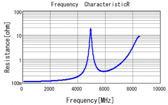
■ GQM1885C2A6R8CB01 R DCOV, 25degC
