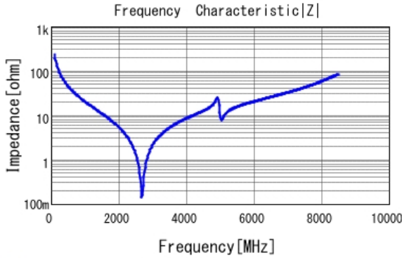
■ GQM1885C2A6R8CB01 |Z| DCOV, 25degC
