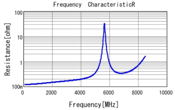
■ GQM1885C2A5R1CB01 R DCOV, 25degC
