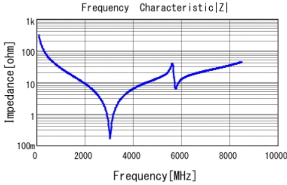
■ GQM1885C2A5R1CB01 |Z| DCOV, 25degC
