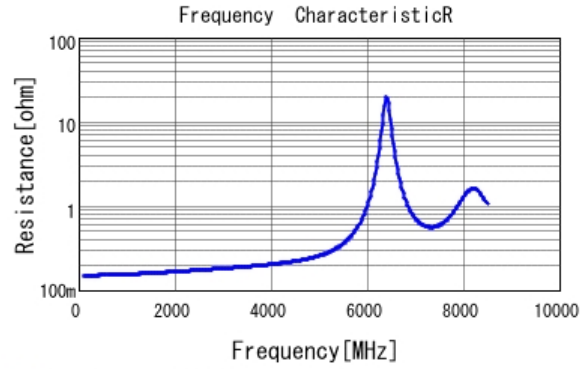
■ GQM1885C2A4R0CB01 R DCOV, 25degC
