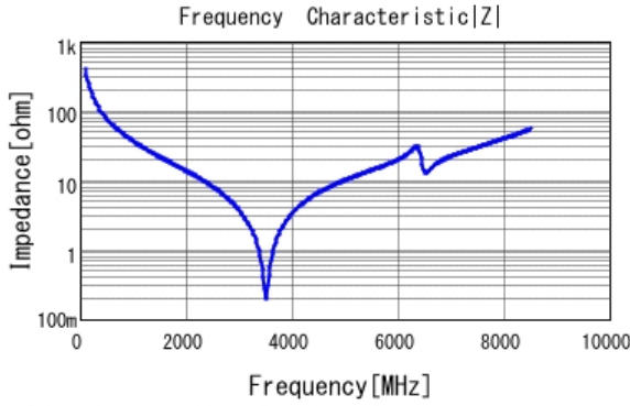
■ GQM1885C2A4R0CB01 |Z| DCOV, 25degC
