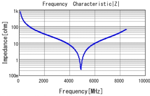
■ GQM1885C2A2R0BB01 |Z| DCOV, 25degC
