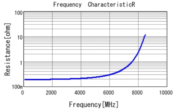
■ GQM1885C2A2R0BB01 R DCOV, 25degC
