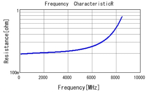
■ GQM1885C2A1R8BB01 R DCOV, 25degC
