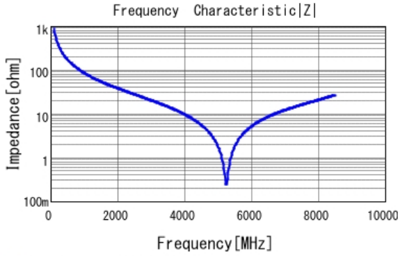
■ GQM1885C2A1R8BB01 |Z| DCOV, 25degC
