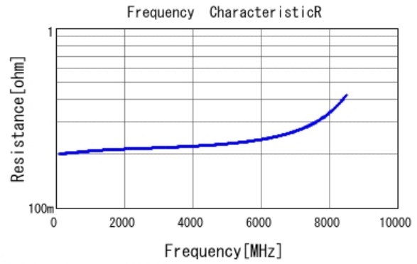
■ GQM1885C2A1R6BB01 R DCOV, 25degC
