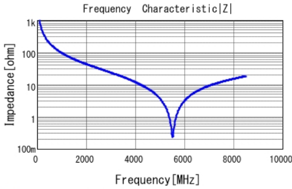
■ GQM1885C2A1R6BB01 |Z| DCOV, 25degC
