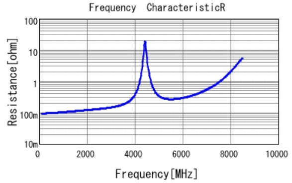
■ GQM1885C1H8R2CB01 R DCOV, 25degC
