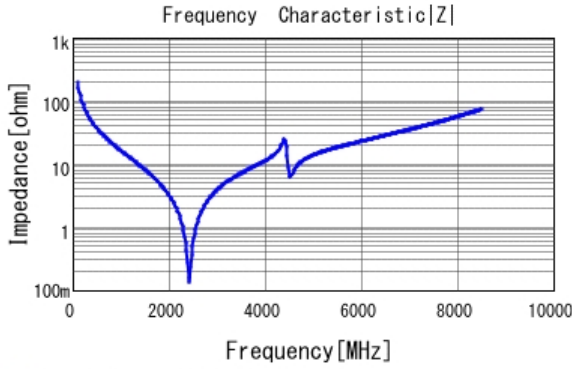
■ GQM1885C1H8R2CB01 |Z| DCOV, 25degC
