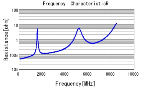
■ GQM1885C1H680JB01 R DCOV, 25degC
