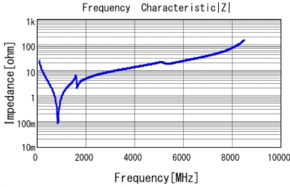
■ GQM1885C1H680JB01 |Z| DCOV, 25degC
